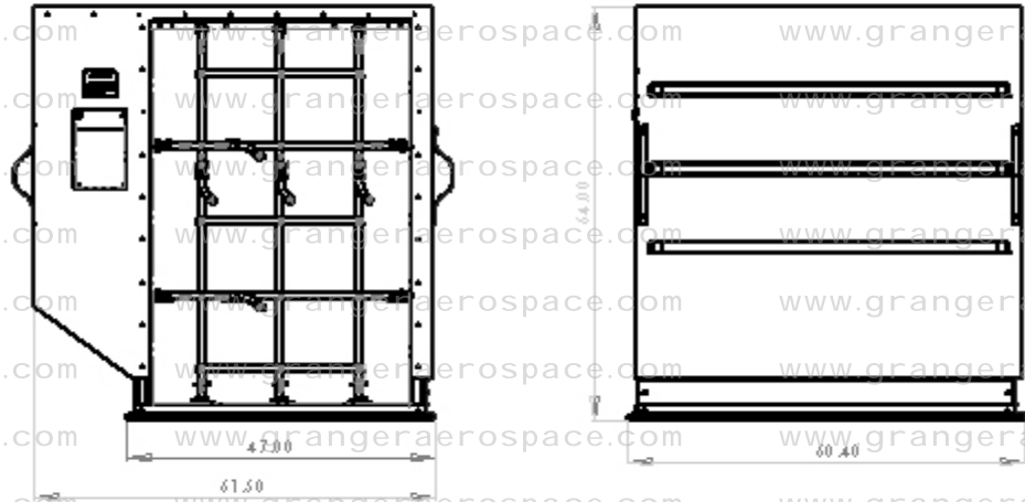
ULD 2 LD 2 Air Cargo Container
